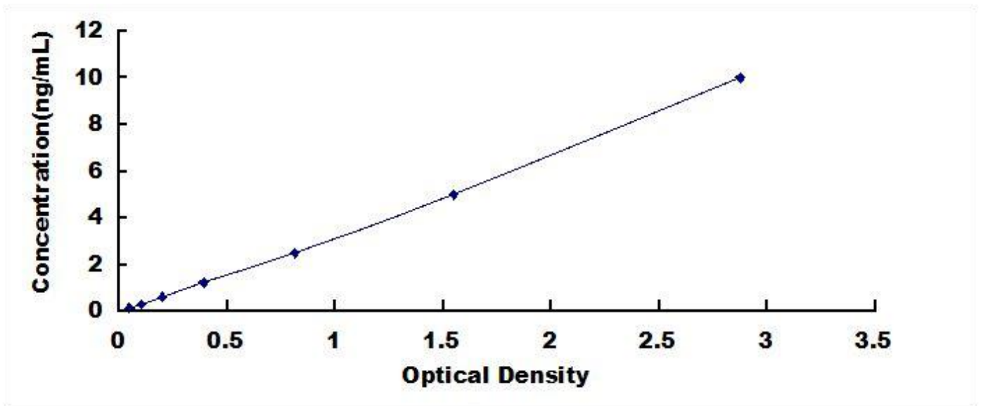
Typical Standard Curve for PRES, Rat ELISA.
