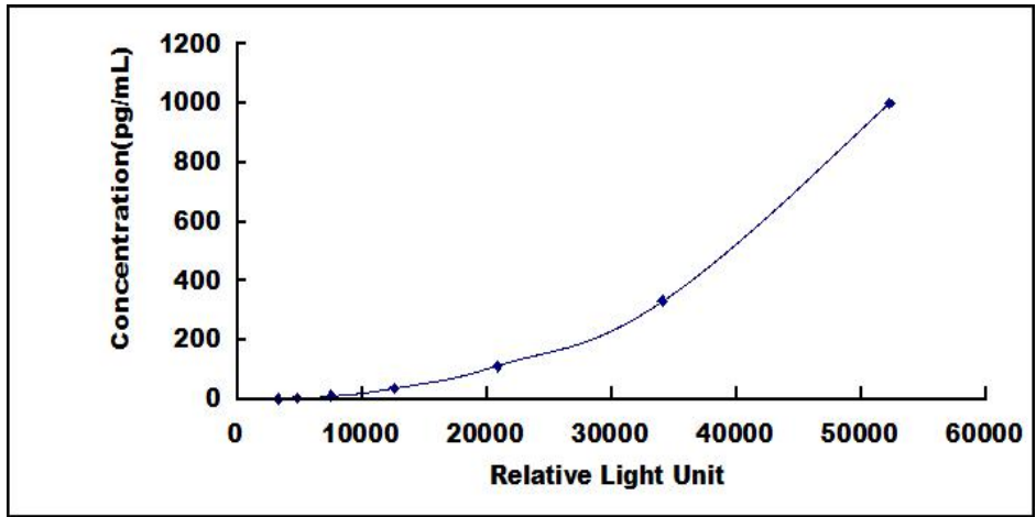
Typical Standard Curve for IL20 ELISA.
