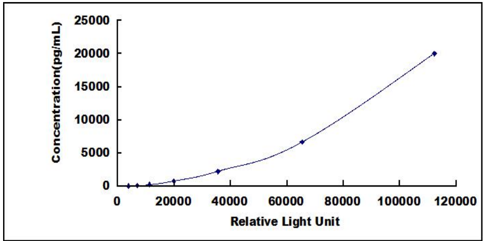
Typical Standard Curve for MMP1 ELISA.
