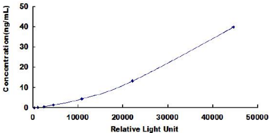
Typical Standard Curve for TFPI ELISA.
