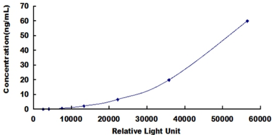
Typical Standard Curve for TIMP3 ELISA.
