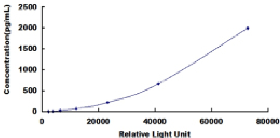
Typical Standard Curve for TGFb1 ELISA.
