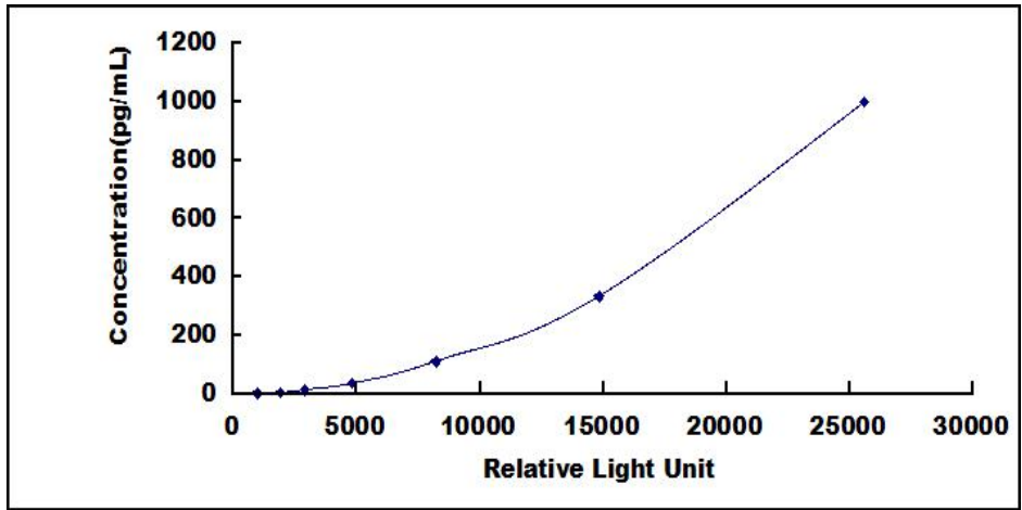
Typical Standard Curve for IL11 ELISA.
