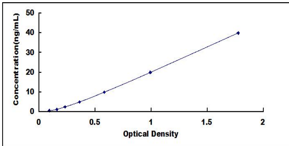
Typical Standard Curve for TRPA1 ELISA.
