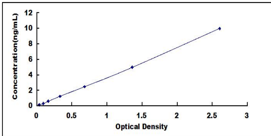
Typical Standard Curve for SSB ELISA.
