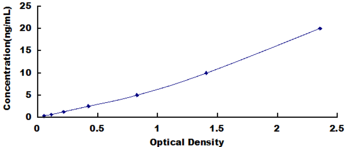
Typical Standard Curve for MYH2, Bovine ELISA.
