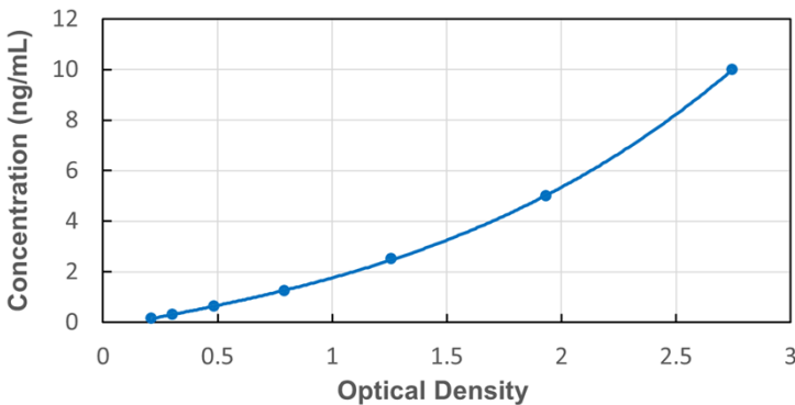
Typical Standard Curve for Human GaA ELISA
