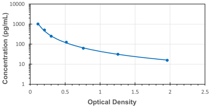
Typical Standard Curve for Mouse SP ELISA
