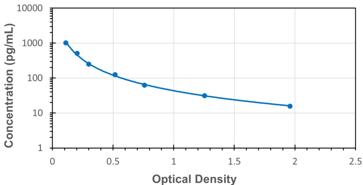
Typical Standard Curve for Human NT-ProCNP ELISA
