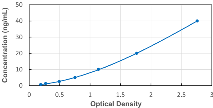
Typical Standard Curve for Human MMP2 ELISA
