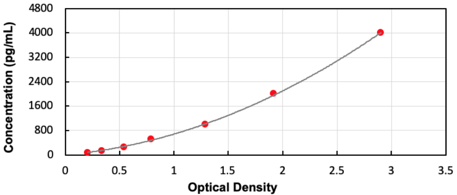
Typical Standard Curve for Human ALDOA ELISA
