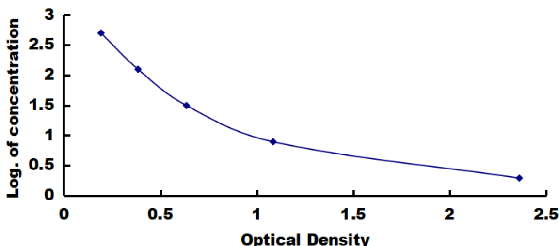
Typical Standard Curve for COL1, Equine ELISA.
