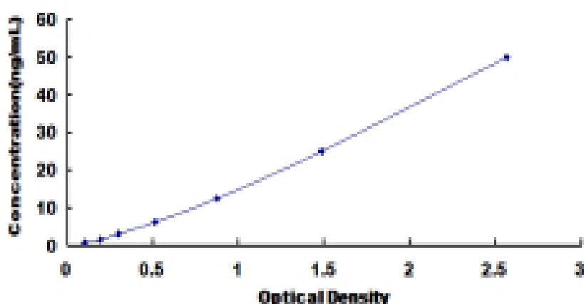
Typical Standard Curve for ALDH2 ELISA.
