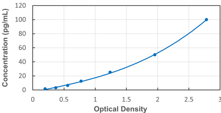
Typical Standard Curve for Human BIN1 ELISA
