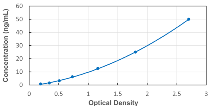
Typical Standard Curve for Human APBB3 ELISA
