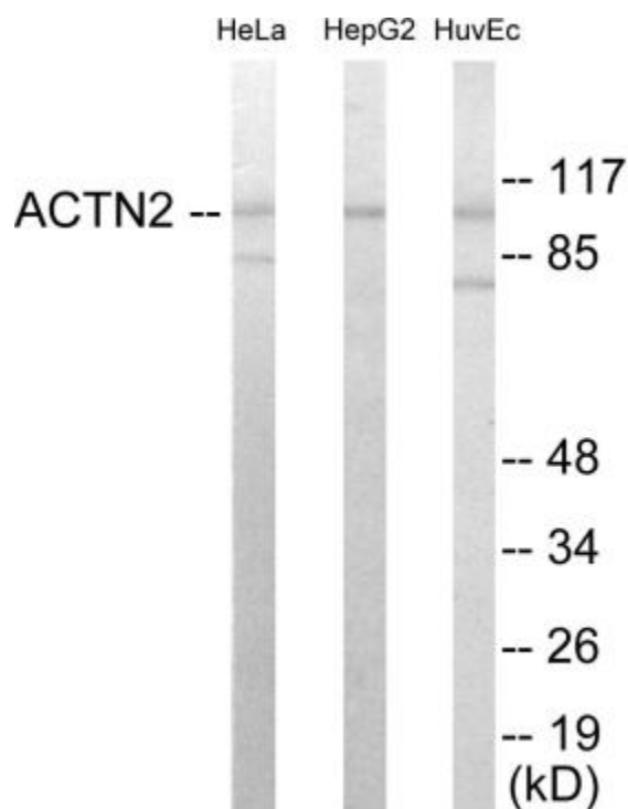
Figure 2. Western blot analysis of extracts from HepG2/HeLa/HuvEc cells, using Actinin alpha-2/3 Antibody.
